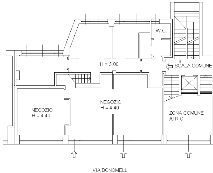
PIANO TERRA
