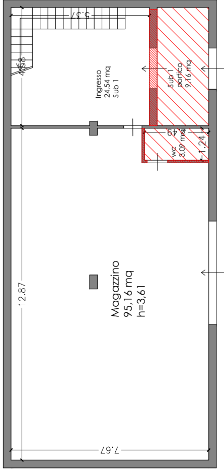
Planimetria piano terra
