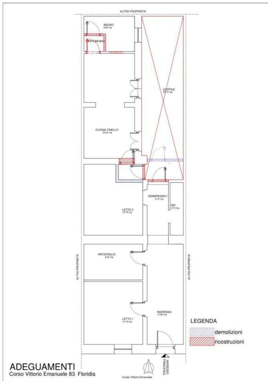
AII.2H_PLANIMETRIA IMMOBILE_ADEGUAMENTI
