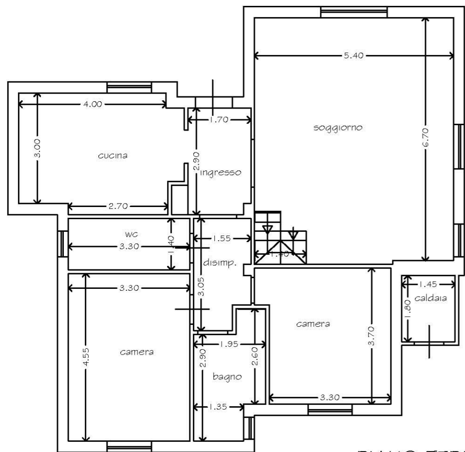
PIANO TERRA
