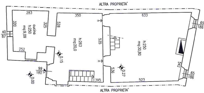
PIANO TERRA
