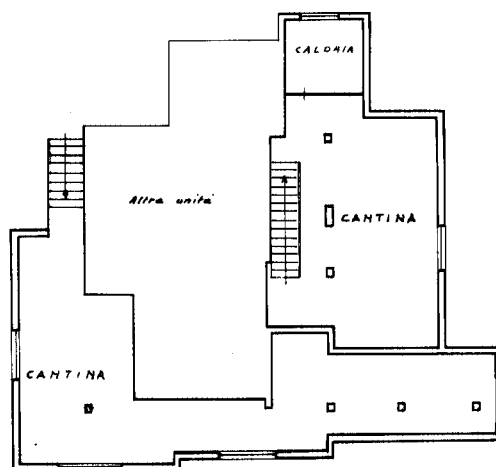
PIANO SEMINTERRATO H: 3.00
