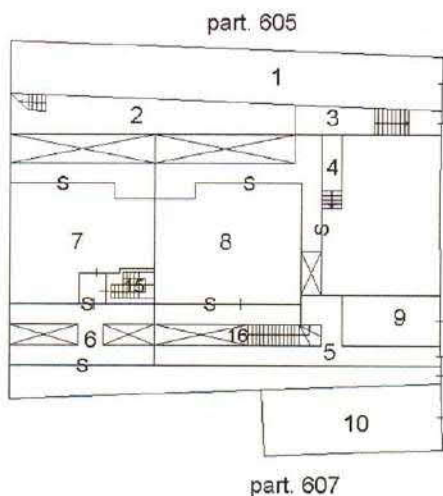
PIANO TERRA
