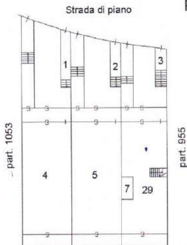
PIANO TERRA
