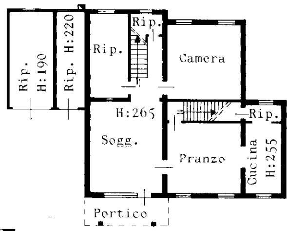
PIANO TERRA
