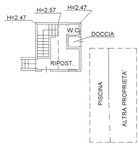
PIANO TERRA
