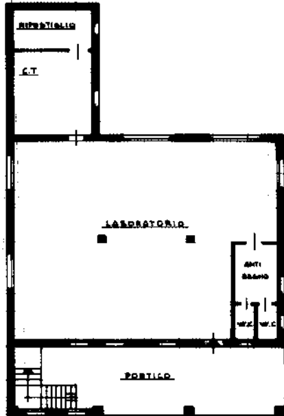
PIANO TERRA H=2.75
