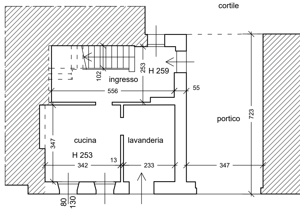
PIANO TERRA
