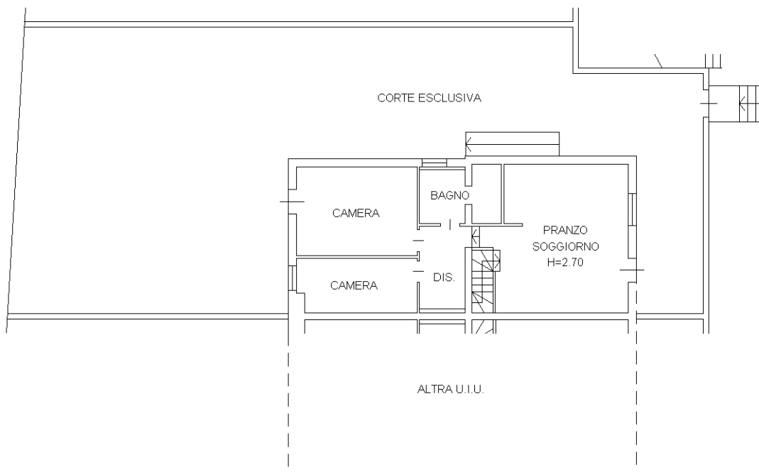
PIANO TERRA
