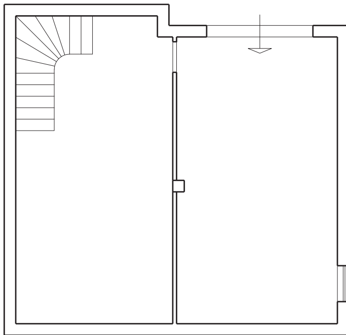
piano seminterrato SCALA 1:100
