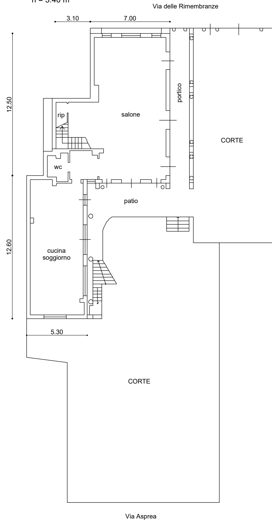
Piano Terra h = 3.40 m
