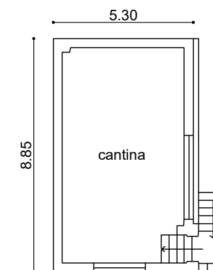
Piano seminterrato h = 2.80 m
