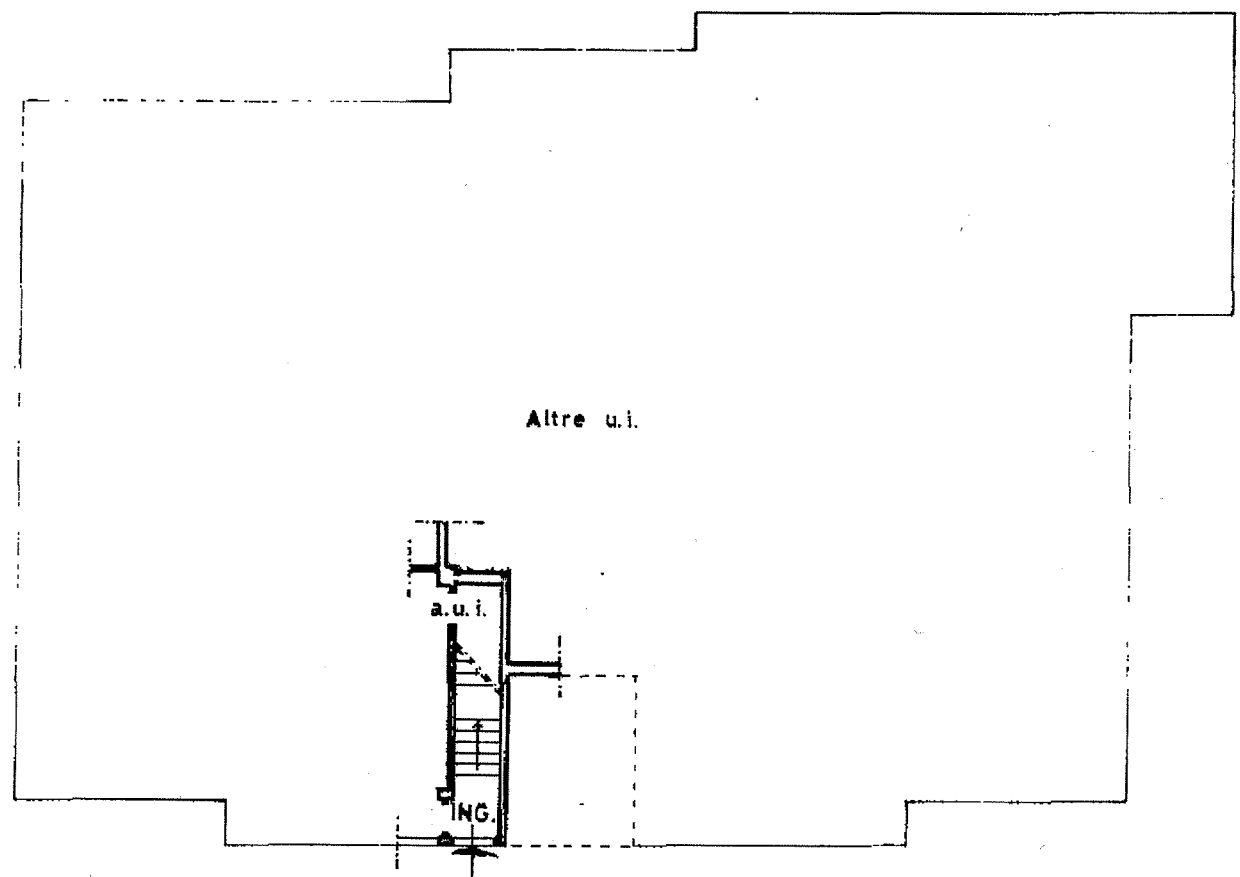
PIANO TERRA
