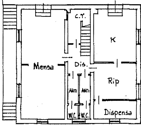
P. Seminterrato h.=300ml.
