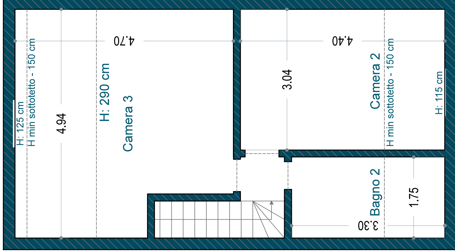
PIANTA REALE PIANO MANSARDA
