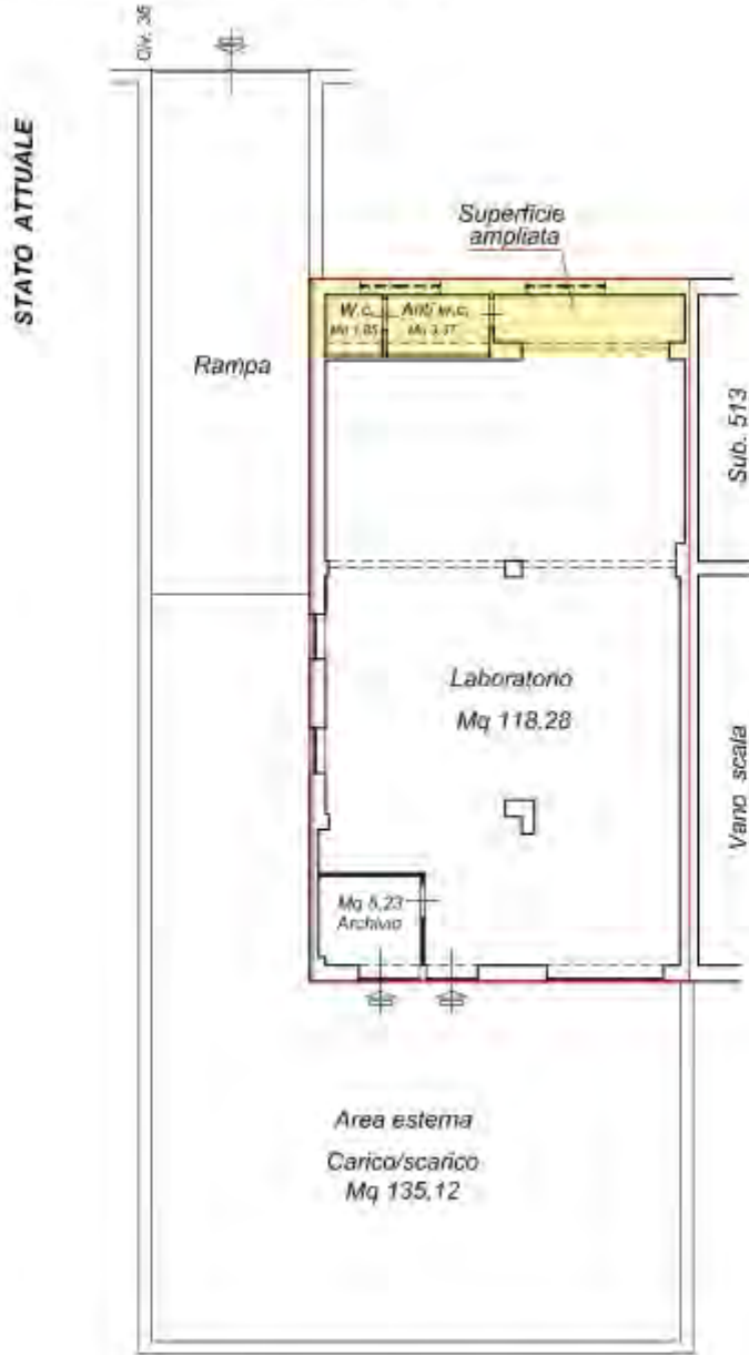
PLANIMETRIA PIANO S1 H = mt 3,00
