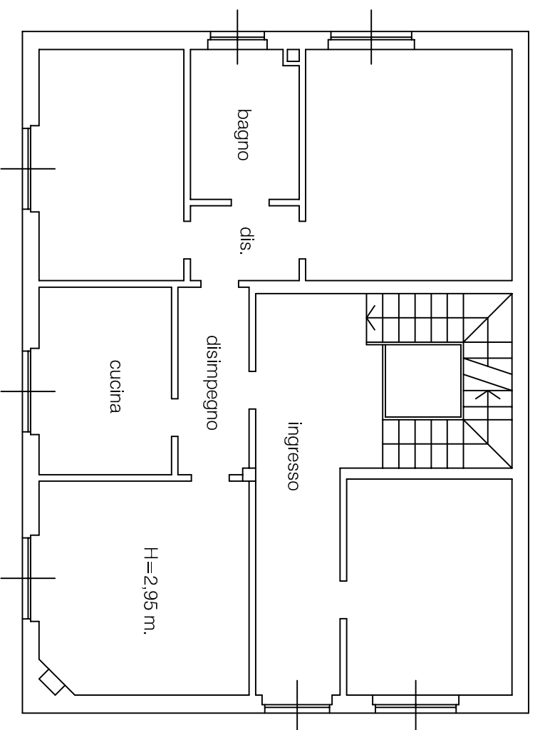
PIANO TERRA
