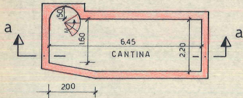
piano interrato
