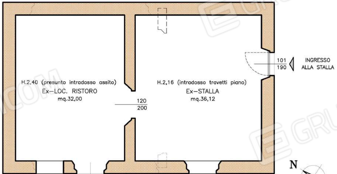
PIANO TERRA
