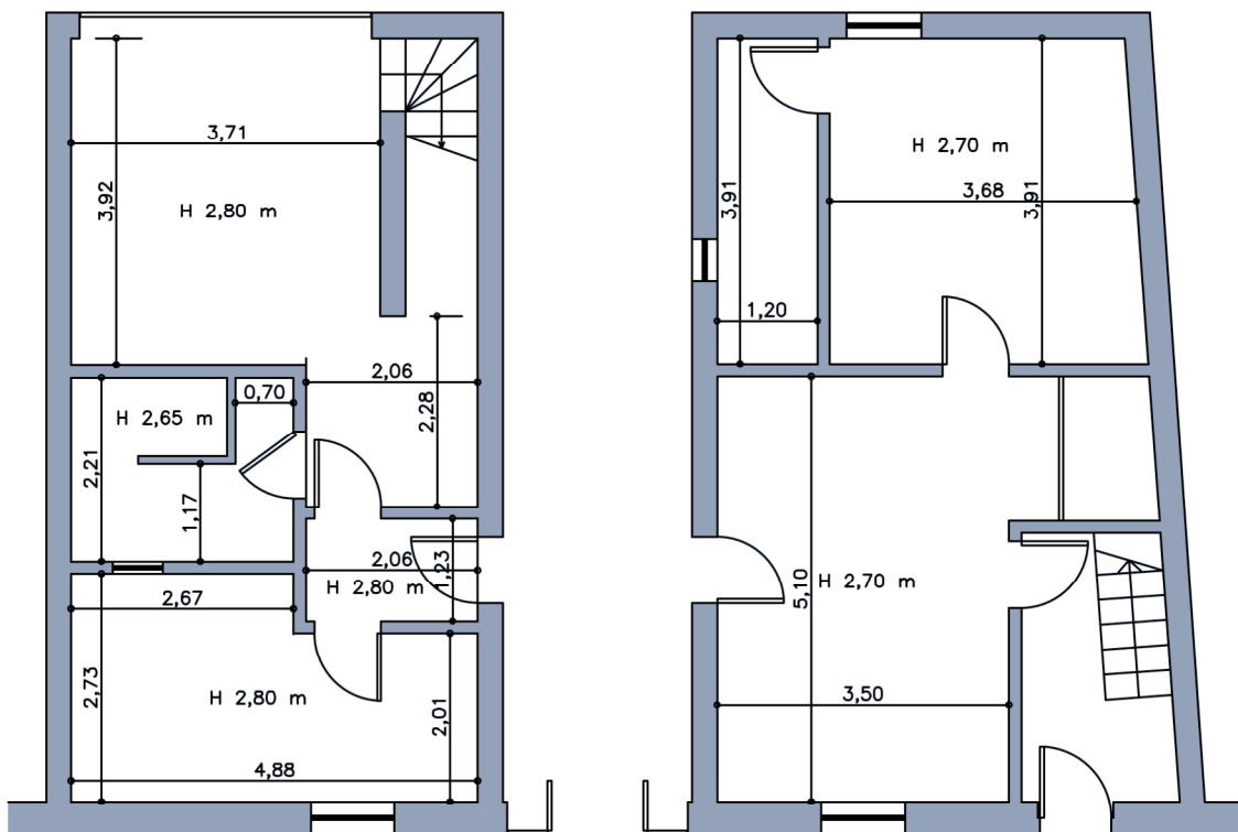
PIANO TERRA
