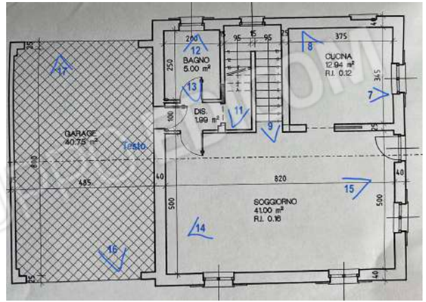
PIANO TERRA
