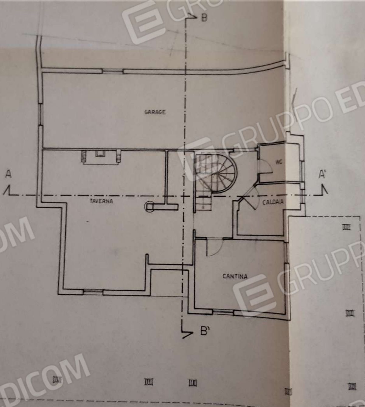
PIANO SEMINTERRATO
