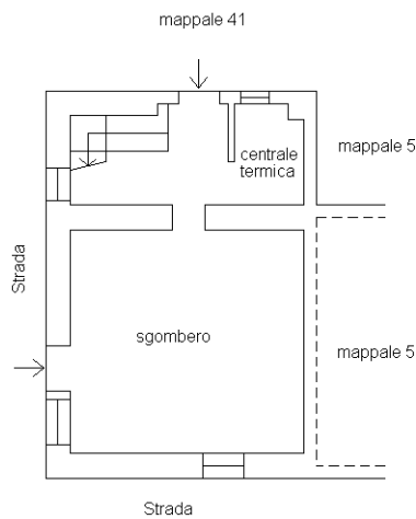
PIANO TERRA h=2.80 mt
